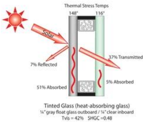
GRAY INSULATED GLASS UNIT
