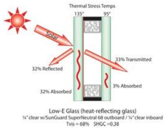
HIGH-PERFORMANCE COATED IG UNIT
