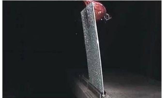
SGP laminated glass impact test
