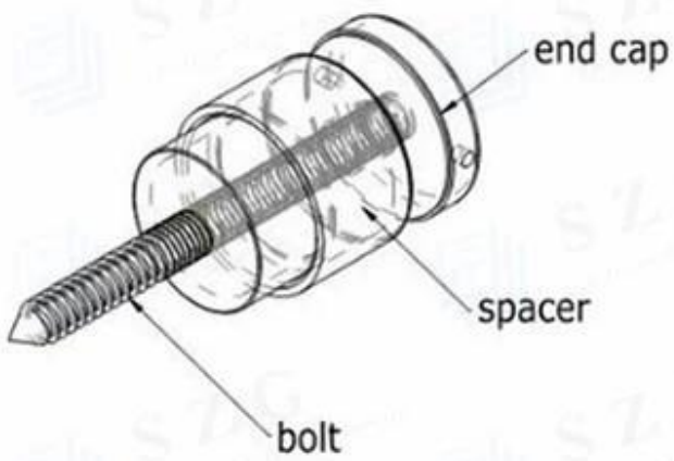
Adjustable glass standoff
